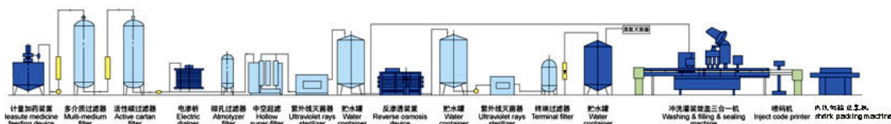
纯净水成套生产设备及工艺 Pure Water Production Line And Production Thnique
