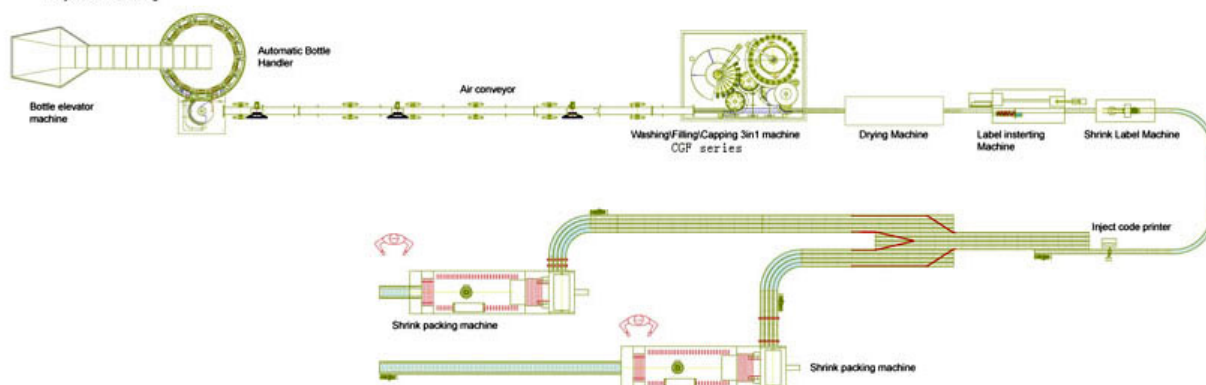
纯净水成套生产设备及工艺 Pure Water Production Line And Production Thnique
