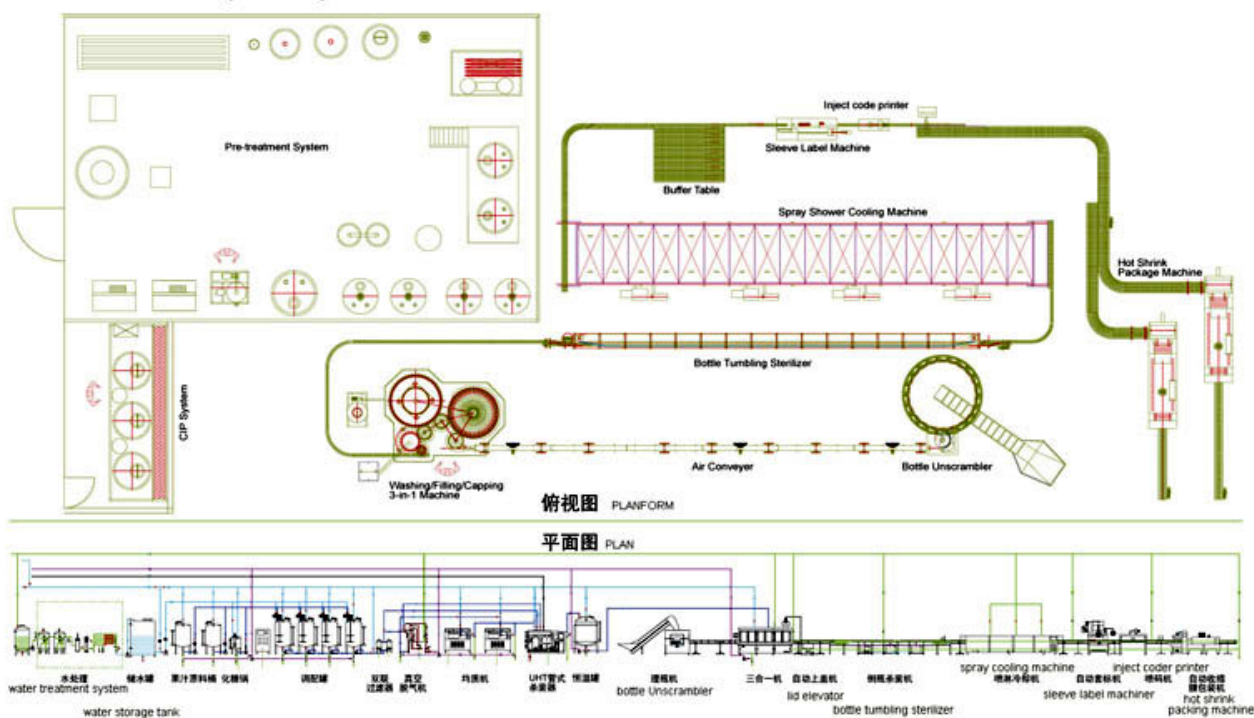
果汁、茶饮料生产车间布置图 Fruit Juice and Tea Drink Layout Drawing
